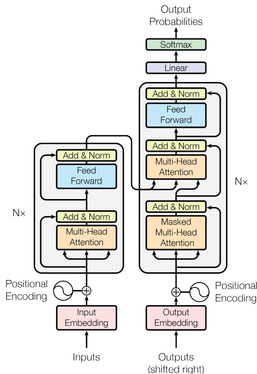
Figure 25: Transformer architecture from [VSP + 23]
