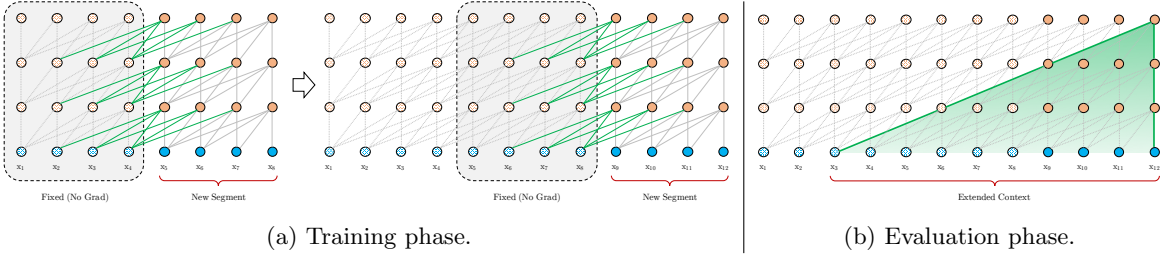
Figure 32: Illustration of the Transformer-XL model with a segment length 4. [DYY + 19]
